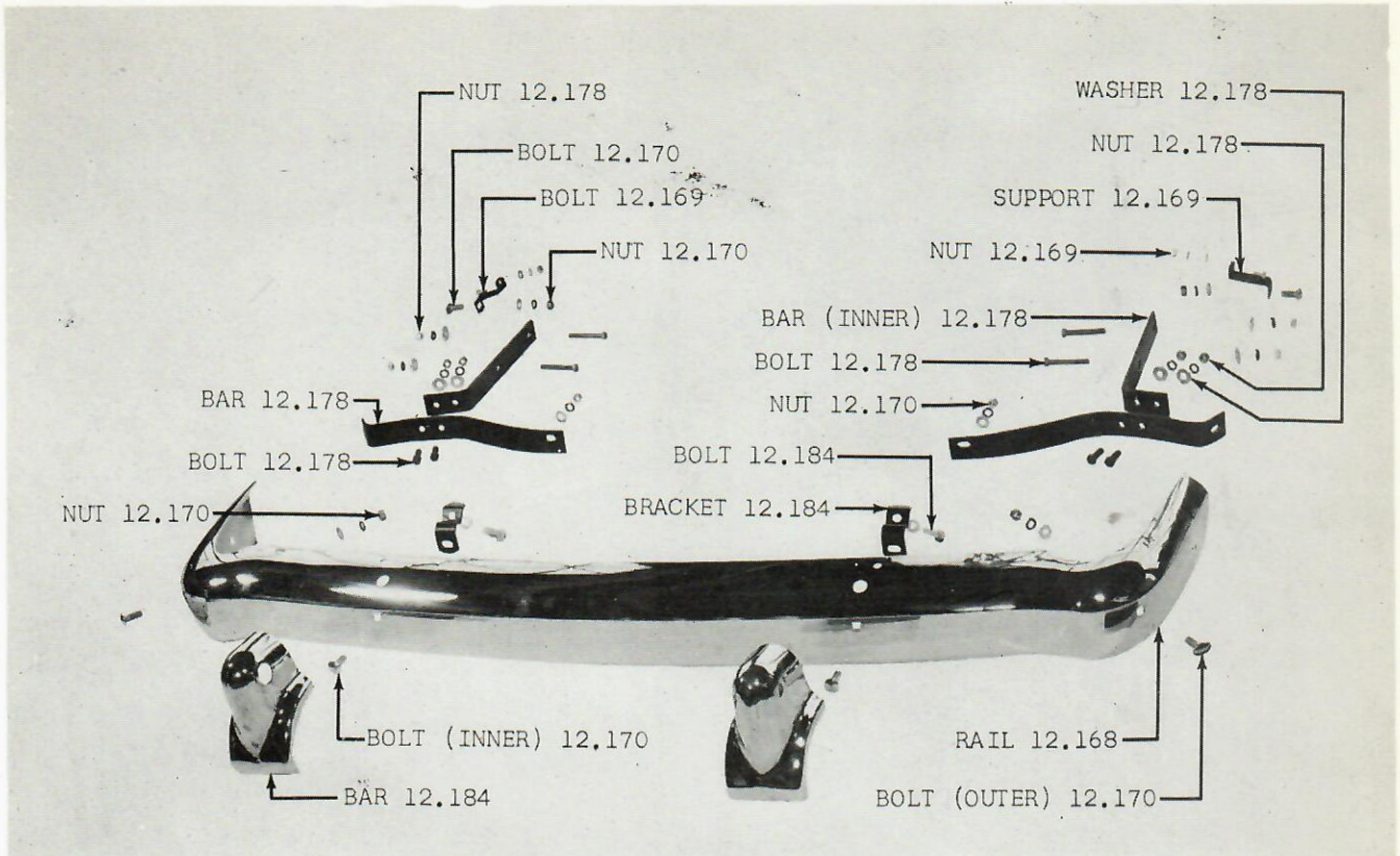
GROUP 12 - FIG. 4 - REAR BUMPER 10-20-80 (LWC)
