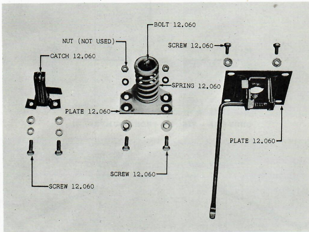
GROUP 12 - FIG. 1 - HOOD LOCK ASSEMBLY 01
