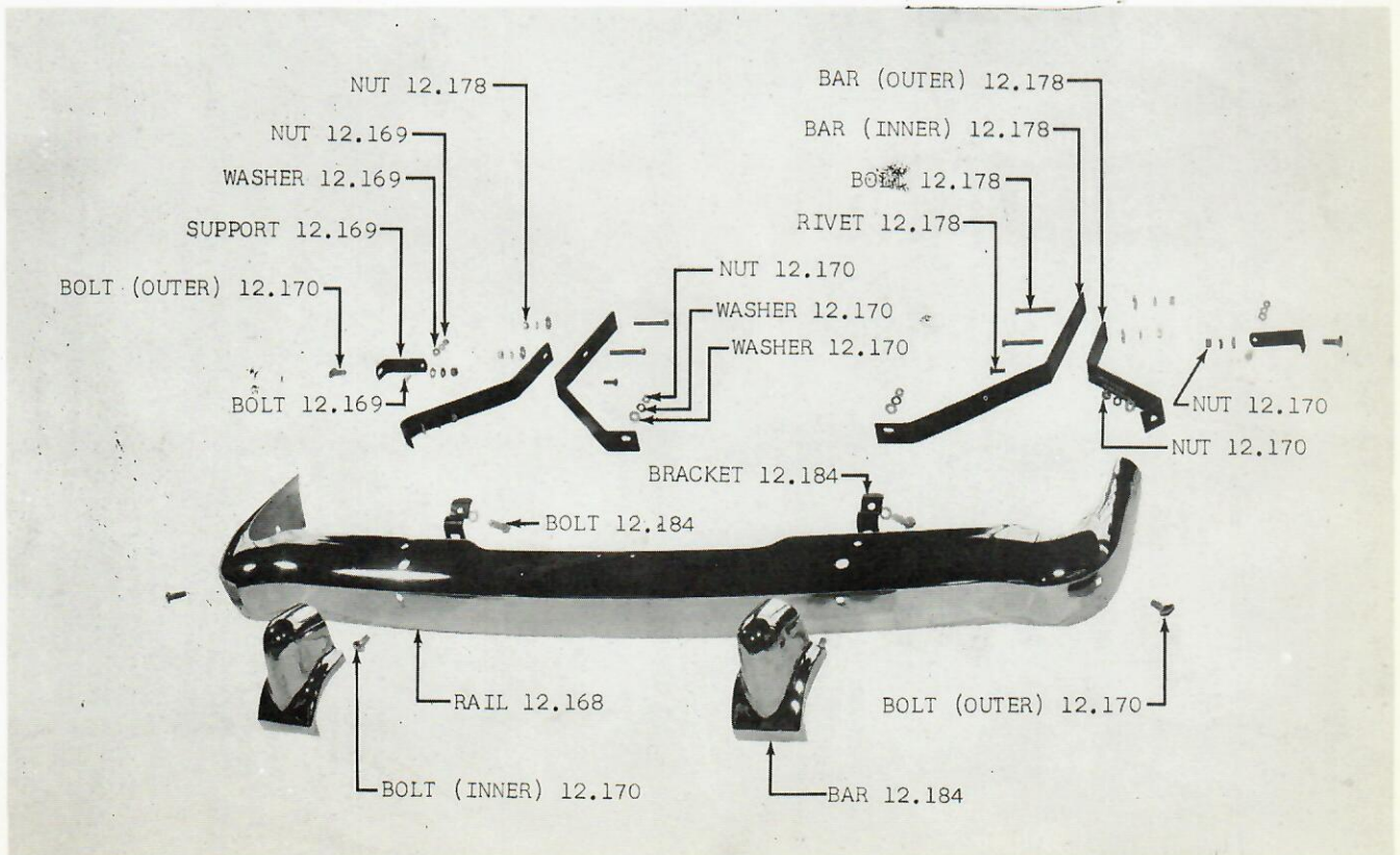
GROUP 12 - FIG. 5 - REAR BUMPER 10-20-80 (WWC)
