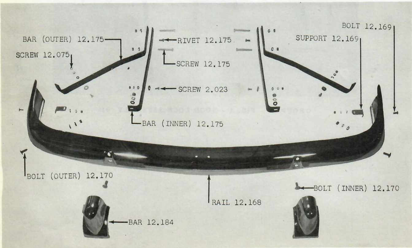
GROUP 12 - FIG. 3 - FRONT BUMPER 10-20-80
